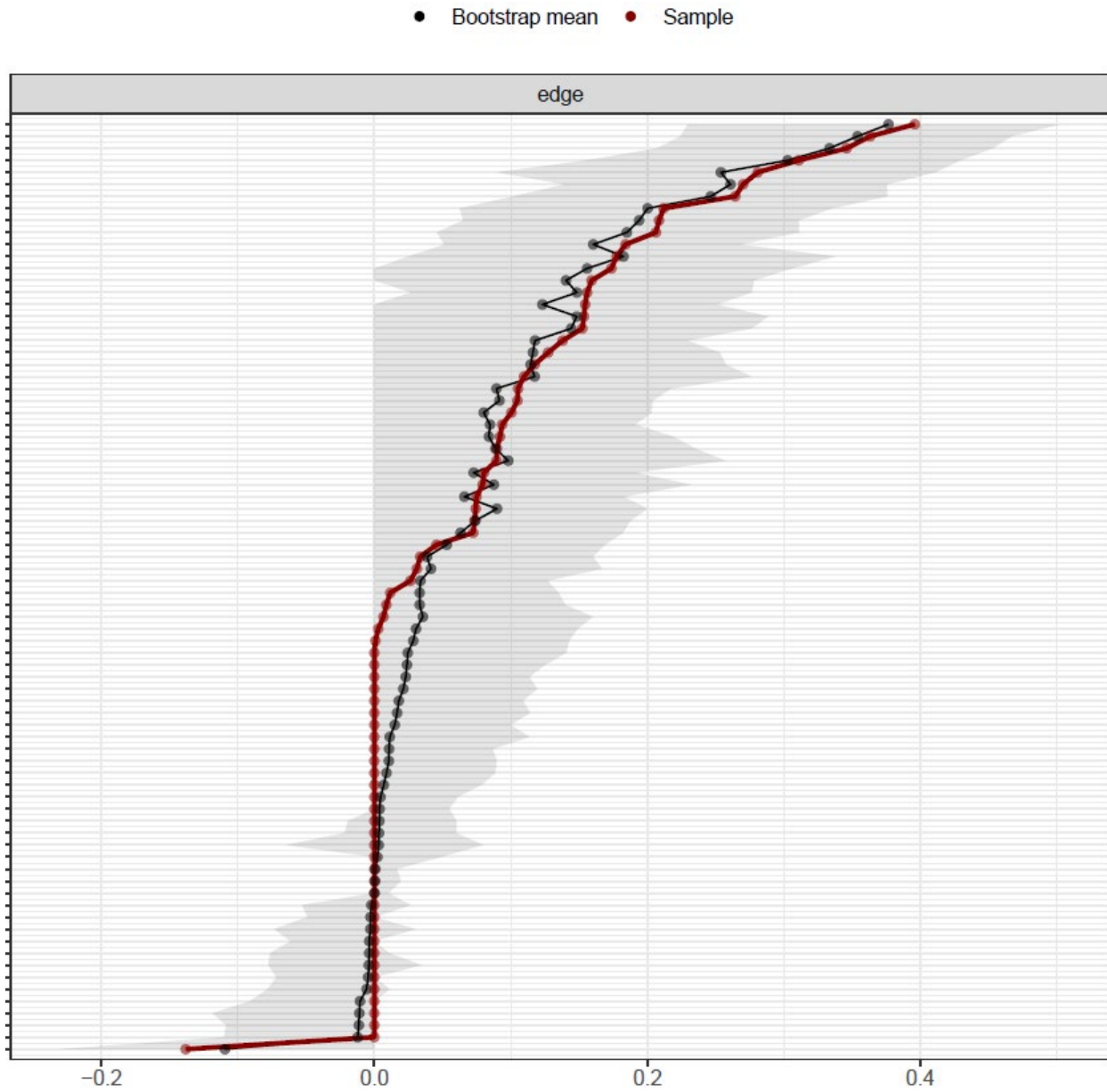
Supplemental Material S1. Edge weights (solid line) and 95% confidence interval (gray bars) around edge weights. Narrower confidence intervals indicate more robust estimation of edge weights.
