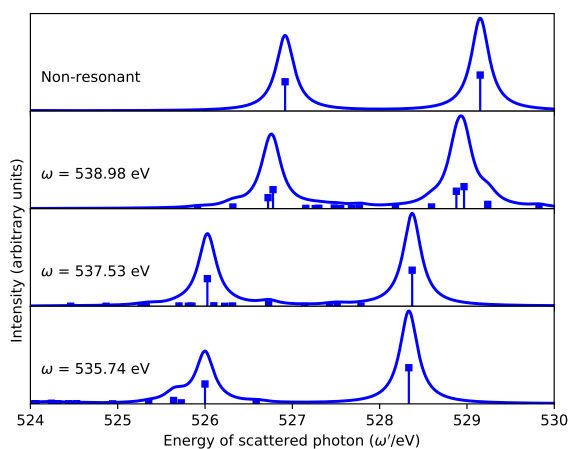
Figure 1: Top: Slices of the core emission spectrum, when the incident beam is at resonance with each of the first few core excited states (RIXS) and when a beam frequency beyond the ionization threshold is used (XES, labeled “Non-resonant”). QR-CCSD/6-311 ++ G ** + (3s,3p)-Rydberg( n=3, 3.5, 4 ) results. The arrows highlight how different states are probed at different resonant frequencies. Bottom left: EOM-CCSD slices of the core emission spectrum. Right: RIXS map, QR-CCSD/6-311 ++ G ** + (3s,3p)-Rydberg( n=3, 3.5, 4 ).
