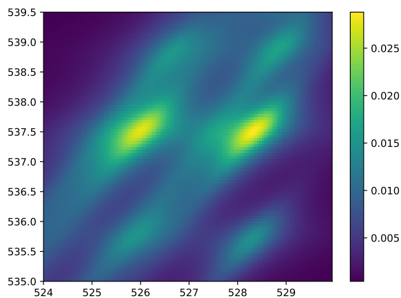
Figure 1: Top: Slices of the core emission spectrum, when the incident beam is at resonance with each of the first few core excited states (RIXS) and when a beam frequency beyond the ionization threshold is used (XES, labeled “Non-resonant”). QR-CCSD/6-311 ++ G ** + (3s,3p)-Rydberg( n=3, 3.5, 4 ) results. The arrows highlight how different states are probed at different resonant frequencies. Bottom left: EOM-CCSD slices of the core emission spectrum. Right: RIXS map, QR-CCSD/6-311 ++ G ** + (3s,3p)-Rydberg( n=3, 3.5, 4 ).
