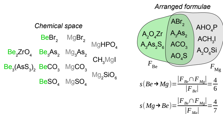
Figure 2: Similarity among chemical elements. A toy-chemical space of 13 formulae. Each formula provides an arranged formula for an element in the given formula. For example, A_2O_4Zr is the arranged formula of Be from formula Be_2ZrO_4 . Arranged formulae of element x are gathered in F_x . Similarity of element x regarding element y is given by s(x \rightarrow y) .
