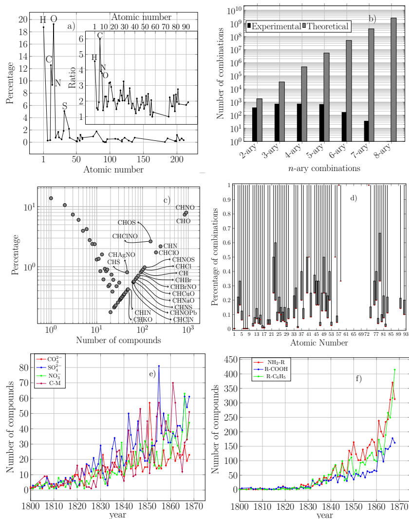
Figure 1: Size and diversity of the chemical space: a) Chemical elements known by 1869 and the percentages of compounds in which they take part. These percentages are non-additive as a single compound adds to each one of its elements, e.g. \text{H}_2\text{O} contributes to both H and O counting. Inset) Ratio between the number of compounds and of combinations for each element. b) Size distribution of combinations. Number of n -ary reported combinations of elements (black) and theoretical bounds (gray) (Methods). c) A pair (x, y) indicates that y = cx percentage of the chemical space is spanned by c combinations accounting for x compounds. d) Box plots of the distribution of compounds per combination for each element, with whiskers indicating combinations with least and most populated compounds; red line shows the median of each distribution. e) Temporal distribution of several typical inorganic, organometallic and f) organic molecular fragments. C-M stands for the bond C-metal, with M = \{\text{Zn}, \text{Sb}, \text{As}, \text{Hg}, \text{Tl}, \text{Bi}, \text{Pb}, \text{Rh}, \text{Co}, \text{Pt}, \text{Li}, \text{Be}, \text{Al}, \text{Fe}, \text{Si}, \text{Ge}\} .
