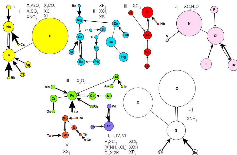
Figure 3: Most similar elements by 1869. Arrows A \rightarrow B indicate that A is most similar to B . Node size is proportional to the number of formulae in which the element represented by the node is involved. Arrow size is proportional to the similarity s(A \rightarrow B) . Shared formulae for elements belonging in a component (connected set of elements) are shown. Formulae of the blue component disregard Zr and Si. Likewise, disulfide of elements in the orange component does not apply to Th and Ce.
