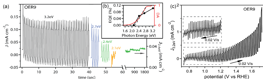
Fig. 2. Summary of toggled illumination PEC experiments on V_2CoO_6 -tri where transition to higher (lower) current corresponds to toggling illumination on (off). (a) CA at 1.23 V vs RHE in pH 9 electrolyte with 4 different light sources (left axis), and an additional 30 min with 2.4 eV illumination where an 11-illumination-cycle moving average of photocurrent is shown (right axis). (b) The corresponding spectral EQE (left axis) along with the UV-vis direct-allowed Tauc plot (right axis). (c) CV with cathodic sweep (inset) starting at 1.23 V vs RHE and anodic sweep extending to 1.73 V vs RHE.
