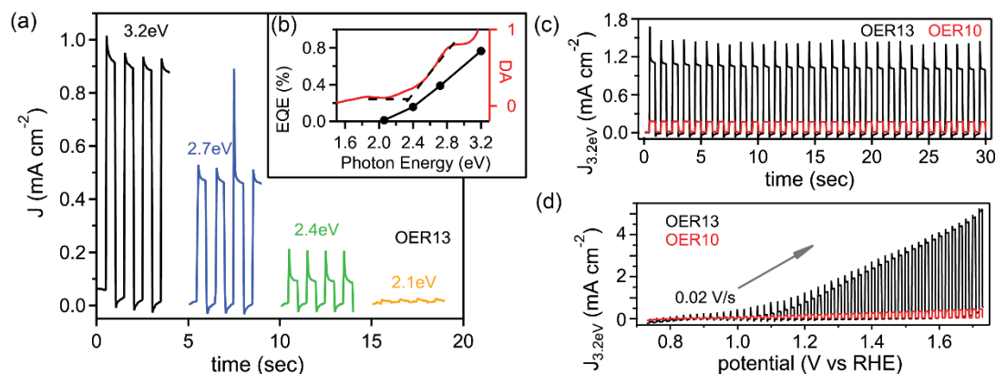
Fig. 1. Summary of toggled illumination PEC experiments on Y_3Fe_5O_{12} where transition to higher (lower) current corresponds to toggling illumination on (off). (a) CA at 1.23 V vs RHE in pH 13 electrolyte with 4 different light sources. (b) The corresponding spectral EQE (left axis) along with the UV-vis direct-allowed Tauc plot (right axis). Nominally duplicate samples were used to compare activity in pH 10 and pH 13 electrolytes, including (c) 30 s CA at 1.23 V vs RHE and (d) CV with 3.2 eV illumination.
