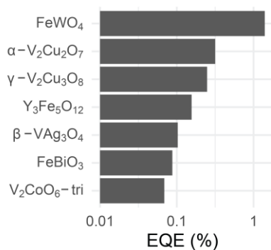
Fig. 3. The top 7 photoanodes by EQE at 2.41 eV from the database of 58 metal oxide photoanode phases (see SI). The photoanodes Y_3Fe_5O_{12} and V_2CoO_6 -tri reported herein are among the most promising phases due to their visible light photoactivity.
