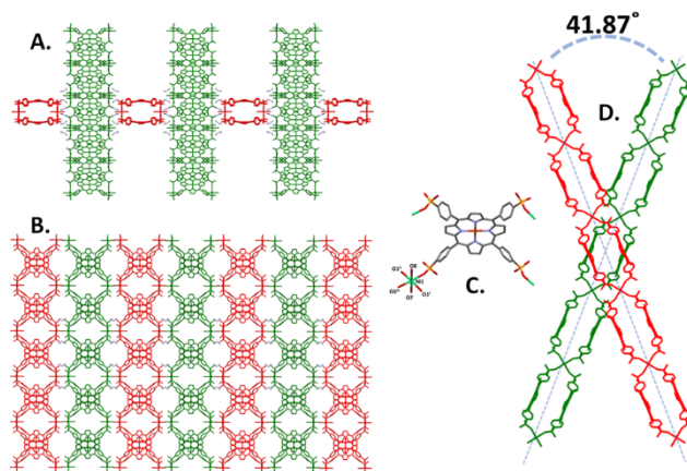
Figure 2. a) b) and d) contain different views of the cross-packed GTUB-4 tubes in the crystal lattice. c) Cu-H_4TPPA^{4+} metal-binding modes with Ni.
