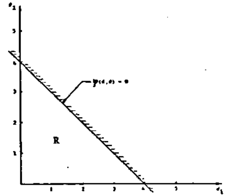
Fig. 7. Plot of region R for the set of constraints in (22) with d = 4 .
