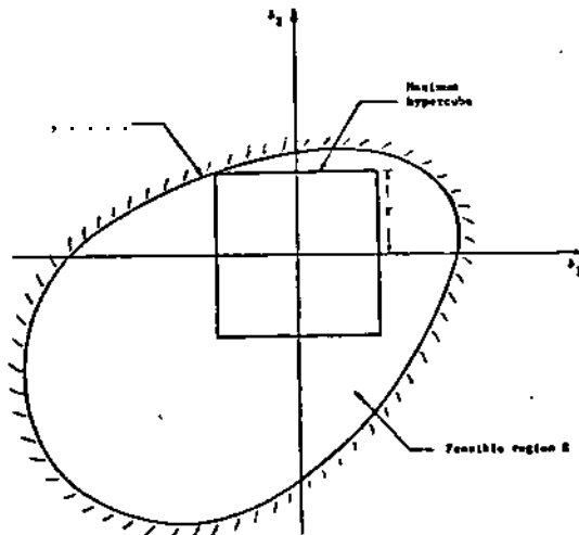
Fig. 8. Maximum hypercube contained in the feasible region R .
