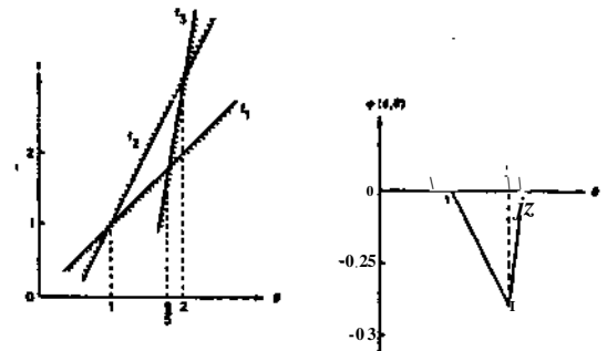
Fig. 2. Feasible region and f(d, \theta) for constraints (16) with d = 1 .
