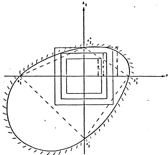
Fig. 10. Lower and upper bounds for maximum hypercube
