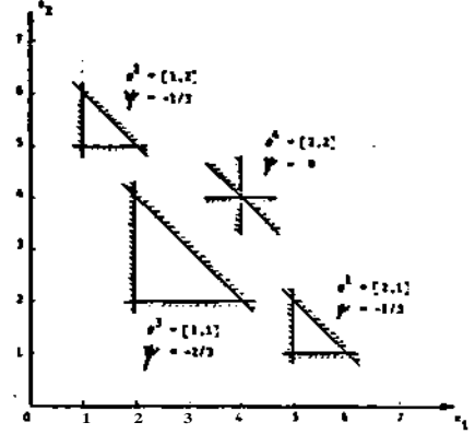
Fig. 4. Feasible region for the constraints in (22) with d = 4 .
