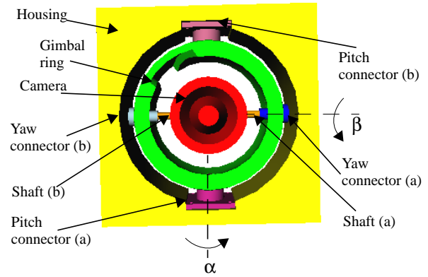
Figure 2: Missile seeker.
