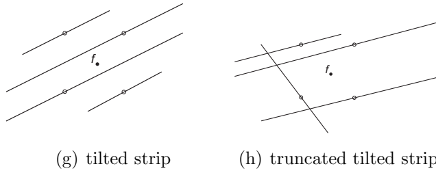
Figure 4: Additional configurations of the parametric octahedron for the 0-1 case
