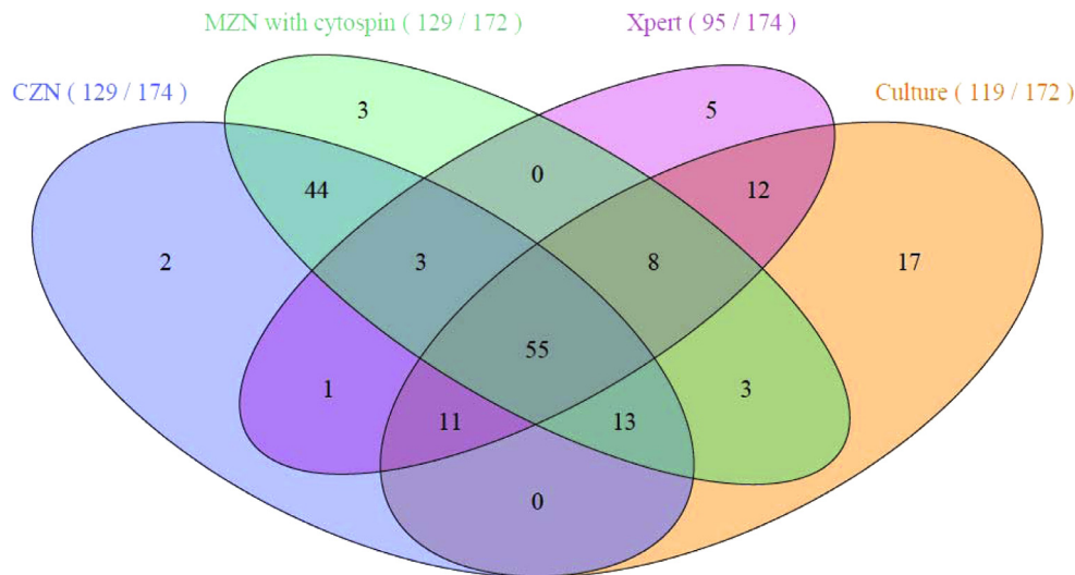
Fig. 2. Venn diagram of mycobacterial tests (conventional ZN, modified ZN with cytospin, Xpert and culture). CZN; conventional Ziehl–Neelsen smear, MZN; modified Ziehl–Neelsen smear, Xpert; Xpert MTB/RIF (Cepheid), culture; mycobacterial culture by MGIT (Becton Dickinson, USA) (Vietnam and South Africa) or MODS (Indonesia). For each test, the number of positive results is shown divided by the number of tests performed. Test denominators (CZN 174, MZN with cytospin 172, Xpert 174, culture 172) refer to the number of definite cases of TBM for which each test was performed.
