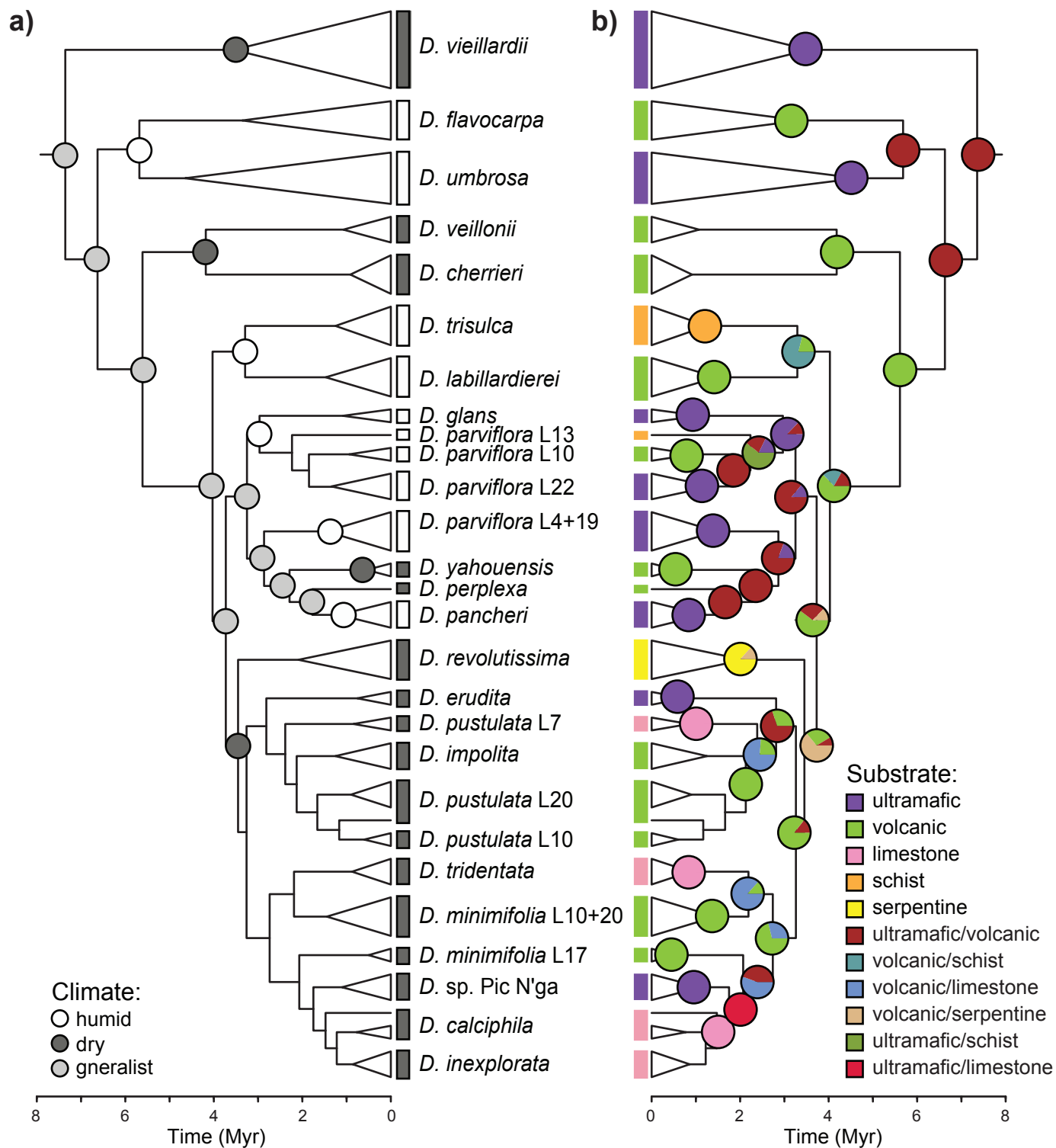
Supplementary Figure 5: Maximum-likelihood reconstruction of habitat evolution for a) climate type and, respectively, b) soil preference. Ancestral conditions are shown at the nodes; current conditions are shown at the tips. Internal nodes without boxes/circles indicate no change in ancestral conditions.
