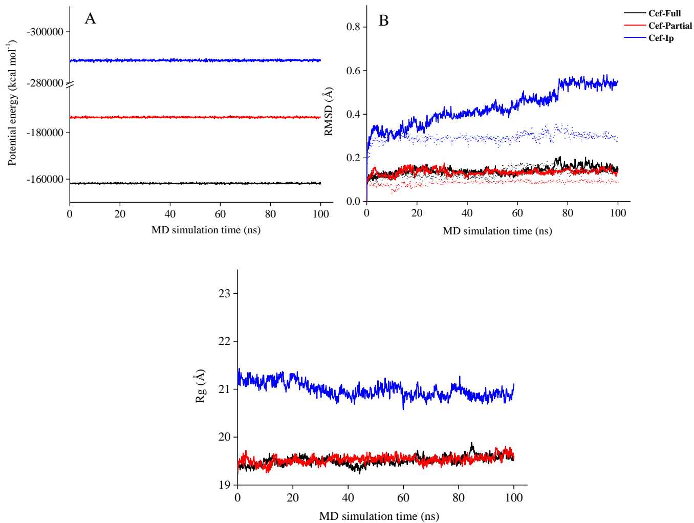
Figure S1. Variation of the potential energy, backbone-atom root-mean-square deviations (RMSD), and backbone radius of gyration (Rg) for various systems during 100 ns molecular dynamics (MD) simulation.
