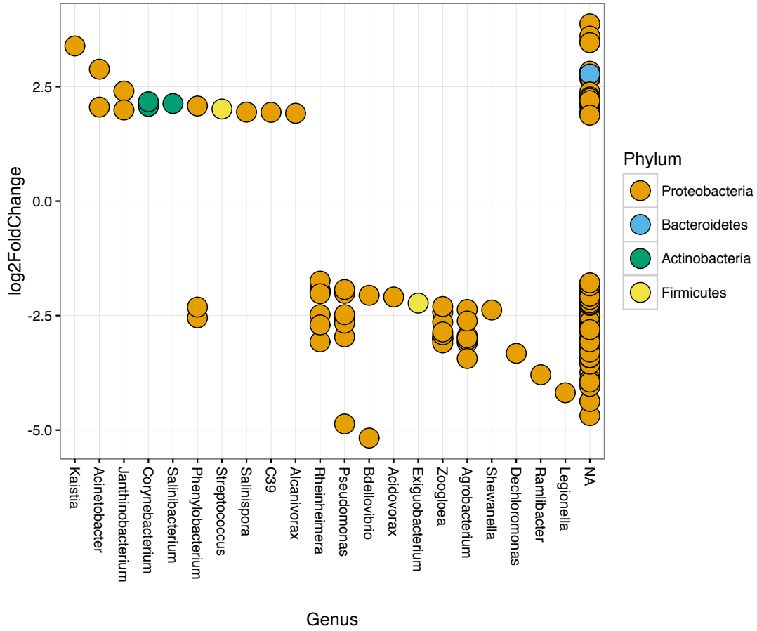
Figure S2. OTUs that significantly differ in abundance in the presence of arsenic. Genus level classification is provided where available. 206 OTUs were identified as significantly different in abundance in the presence of arsenic (DESeq2; adj- P_s \leq 0.01 ).
