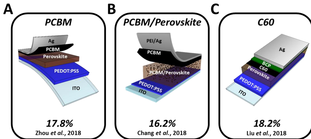
Supplementary Figure 2. Schematic diagram and corresponding PCE of p-i-n perovskite device with different EEL. (A) PCBM, (B) PCBM/perovskite BHJ, and (C) C60.
