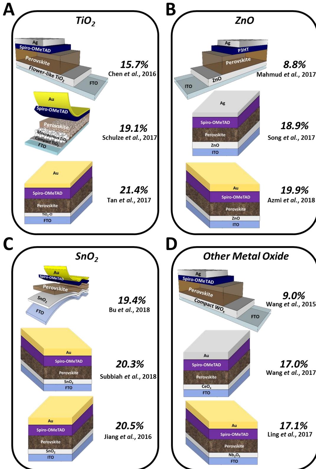
Supplementary Figure 1. Schematic diagram and corresponding PCE of n-i-p perovskite device with different EEL. (A) TiO_2 , (B) ZnO , (C) SnO_2 , and (D) other metal oxide.
