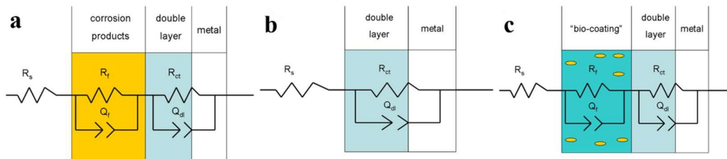
Supplementary Figure 2. Equivalent circuits used for simulate experimental impedance diagrams for the coupons in medium with (a) only V. natriegens and (b) co-cultures of V. natriegens and B. subtilis (before day 7) (c) co-cultures of V. natriegens and B. subtilis (day 9).
