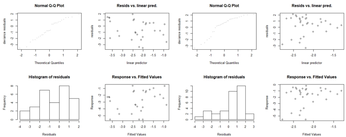
Supplementary Figure 5 - Residuals ( $gam.check ) of spatio-physical models (for each response variable (in order from top to bottom: live hard coral, dead hard coral, branching morphologies, encrusting morphologies, massive morphologies, CCA, macroalgae, turf algae). Left set of graphs = models based on low local impact sites (< 25 humans km -2 reef); right set of graphs = models based on high local impact reefs (> 25 humans km -2 reef):
