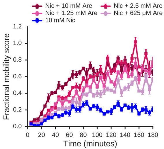
Figure S5: Further characterization of mAChR recovery
