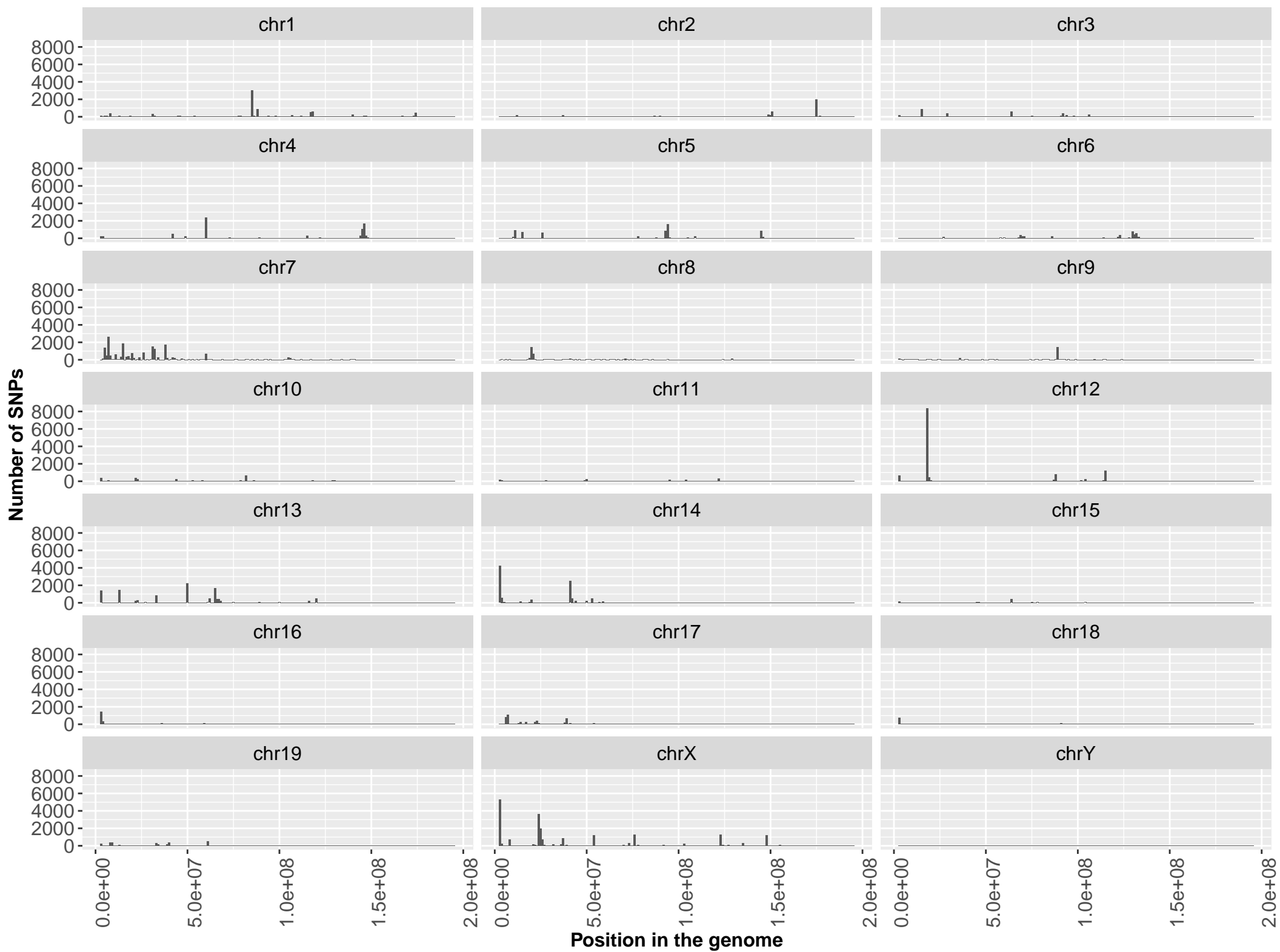
Position of SNPs Resulting from B6Eve Illumina Mapping to B6Eve Assembly
