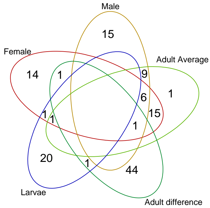
Figure S5 Venn diagram showing the overlap of target genes between all adult and larval phenotypes.
