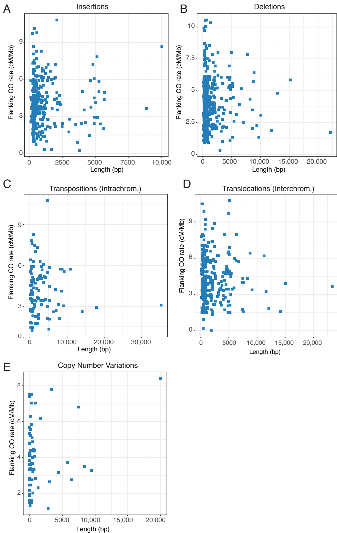
Figure S9. Mean CO rates in the 200-kb up- and downstream of structural variants. Linear regressions revealed a significant correlation between variant size and the mean flanking CO rates only for copy number variations ( p = 0.05 with an R^2 value of 0.05).
