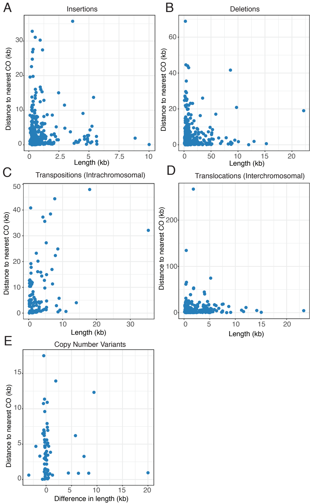
Figure S7. Distance to nearest crossover position from the borders of structural variants as a function of the size of the variant region. Linear regressions revealed no significant correlation between variant size and the distance to the nearest CO position for any of the variants shown in the plots.
