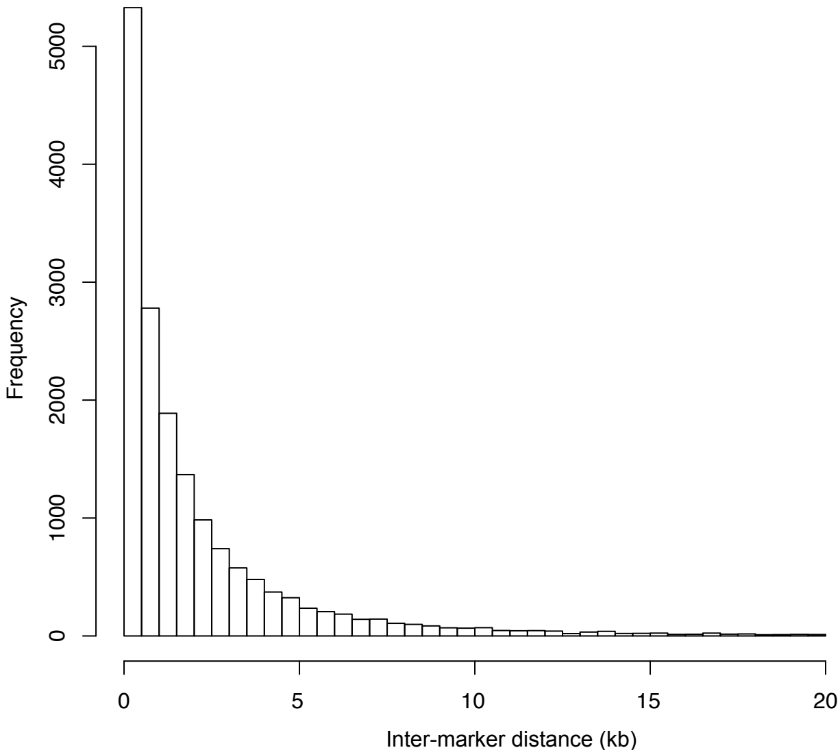
Figure S3. Crossover resolution. The interval window for CO breakpoint estimation (calculated by the distance between flanking markers determined by TIGER). Shown are the intervals for 16,709 of 17,077 total COs, as intervals > 20 kb have been omitted for ease of visualization.
