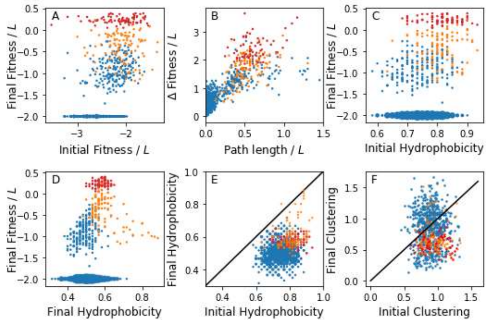
Figure S1: Adaptive origin-fixation evolution from randomly-generated initial sequences to a local peak on the fitness landscape \bar{F}(x) , identical to Fig. 2 except with \alpha = 2.0 .
