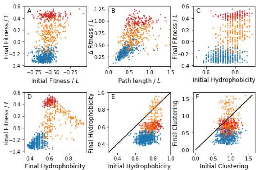
Figure S2: Adaptive origin-fixation evolution from randomly-generated initial sequences to a local peak on the fitness landscape \bar{F}(x) , identical to Fig. 2 except with \alpha = 0.5 .
