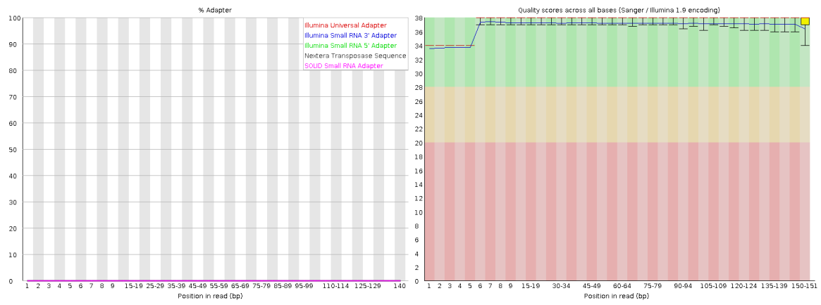
Figure S1: Quality control checks of the raw read data using FastQC. No adapters were present (left) and base quality scores were >30 , equivalent to an error rate of <0.1\% (right).
