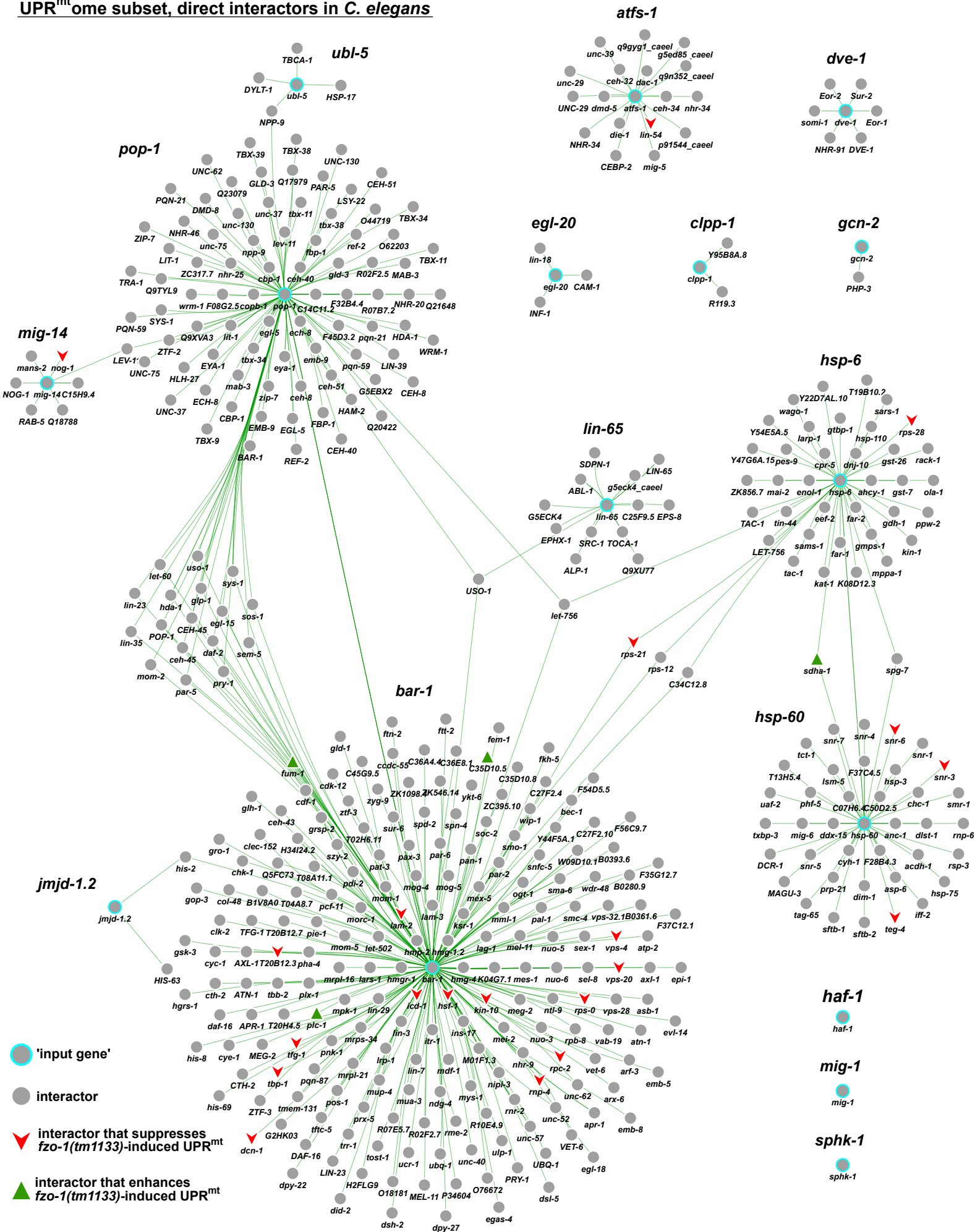
Figure S4: Subset of the UPR mt ome, direct interactors in C. elegans . 'Input genes' associated with the GO-term 'mitochondrial unfolded protein response' are indicated by turquoise circles and their interactors in C. elegans are indicated by grey dots. Red arrowheads: suppressors of fzo-1(tm1133) -induced UPR mt that overlap with the UPR mt ome subset; Green triangles: enhancers of fzo-1(tm1133) -induced UPR mt that overlap with the UPR mt ome subset.
