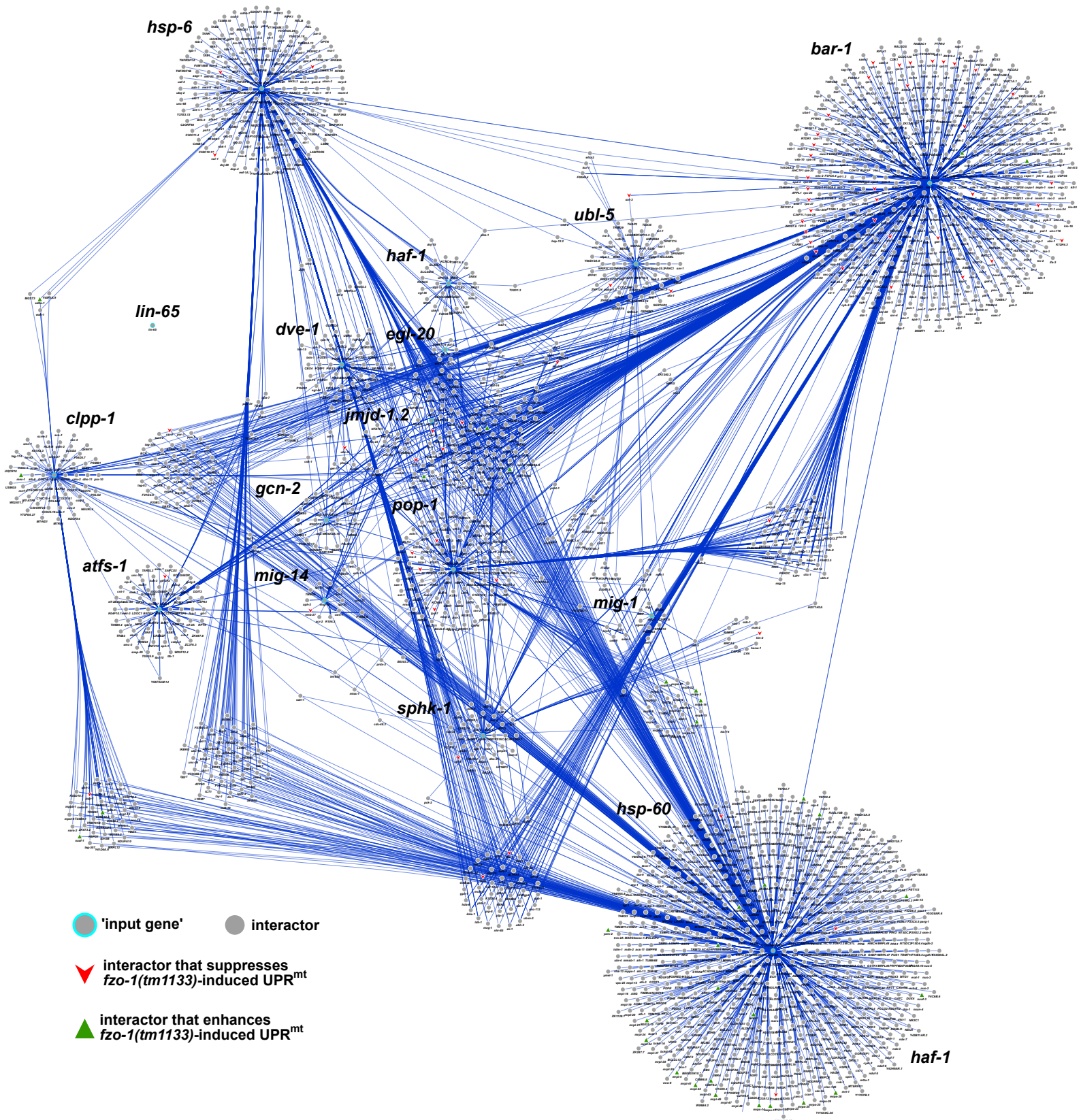
Figure S5: Subset of the UPR mt ome, interactors of human orthologs. 'Input genes' associated with the GO-term 'mitochondrial unfolded protein response' are indicated by turquoise circles and their interactors in humans are indicated by grey dots. Red arrowheads: suppressors of fzo-1(tm1133) -induced UPR mt that overlap with the UPR mt ome subset; Green triangles: enhancers of fzo-1(tm1133) -induced UPR mt that overlap with the UPR mt ome subset.
