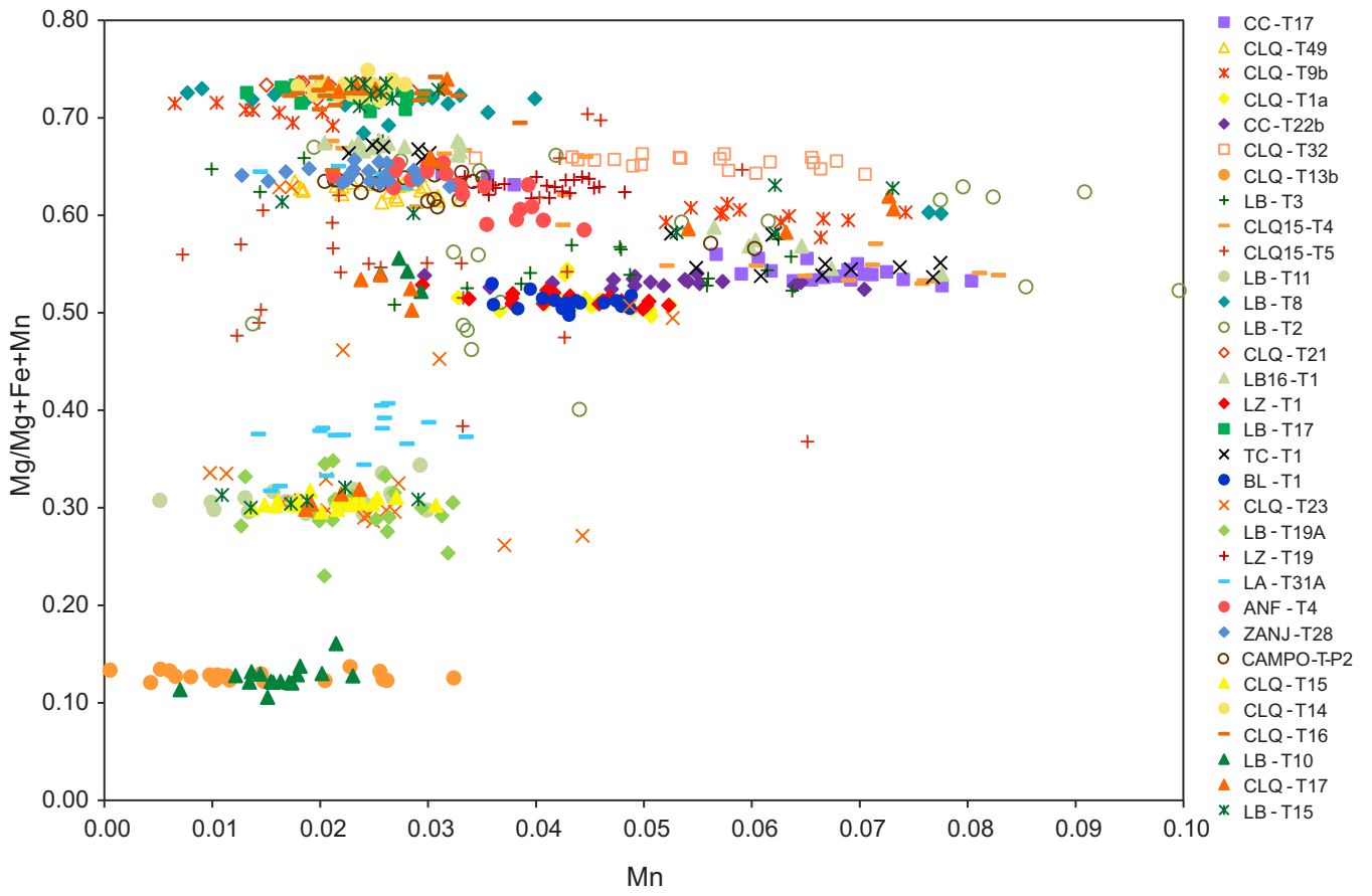
Fig. S4. Biotite Mg/Mg+Fe+Mn vs Mn diagram of P2 ash layers. Values shown as atoms per formula unit.
