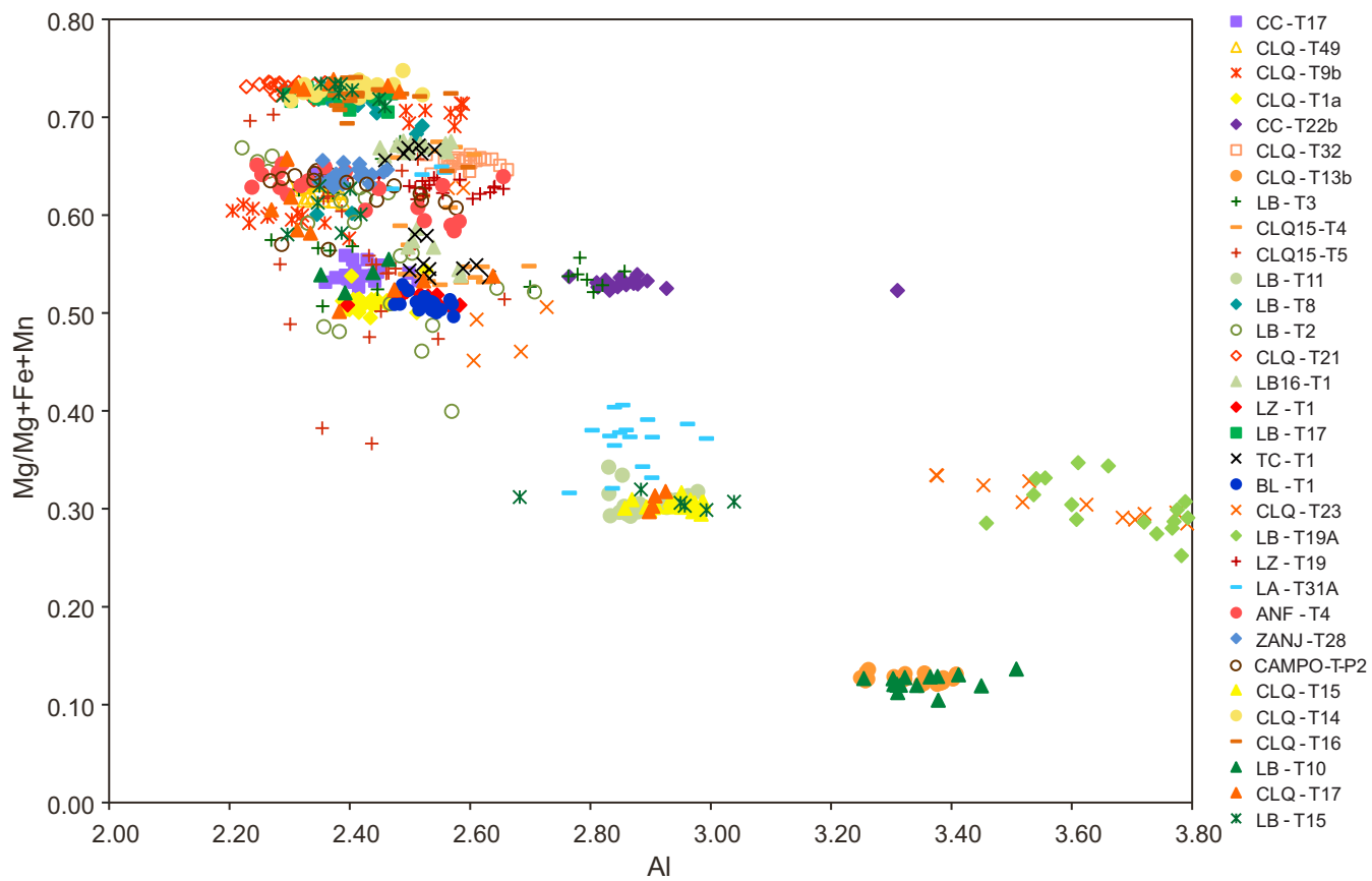
Fig. S3. Biotite Mg/Mg+Fe+Mn vs Al diagram of P2 ash layers. Values shown as atoms per formula unit.
