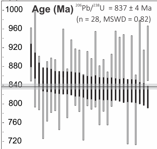
(h) Mr15-04: Tonalite
