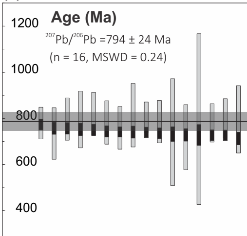
(e) AJ14-25: Granite
