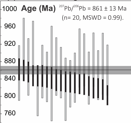
(g) Mr15-02: Tonalite
