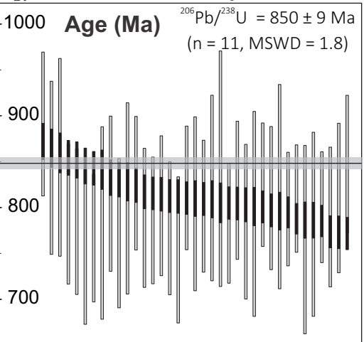
(j) Mr15-07: Sath Complex
