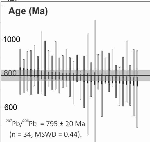
(j) Mr15-07: Sath Complex
