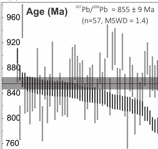
(f) Mr15-01: Mirbat Granite
