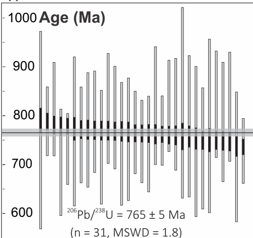
(i) Mr15-05: Monzonite
