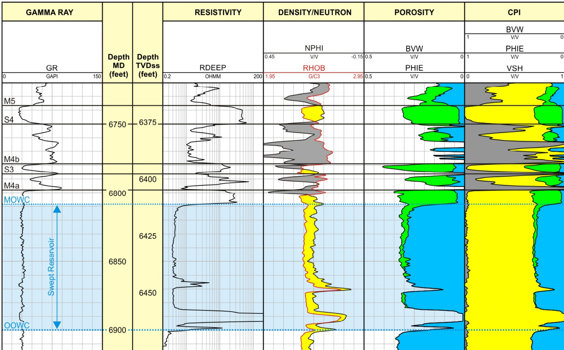
Supplementary material 6. Wireline log character in well 15/20a-18 across the Lower Balmoral Sandstone Unit. This well was drilled following several years of production from the Donan Field redevelopment. In the interval interpreted to be swept, S_w is considerably higher than calculated in the elevated S_w intervals. Additionally, the character of the logs is inconsistent with those recorded in the elevated S_w intervals (after Ings et al. 2015 ).
