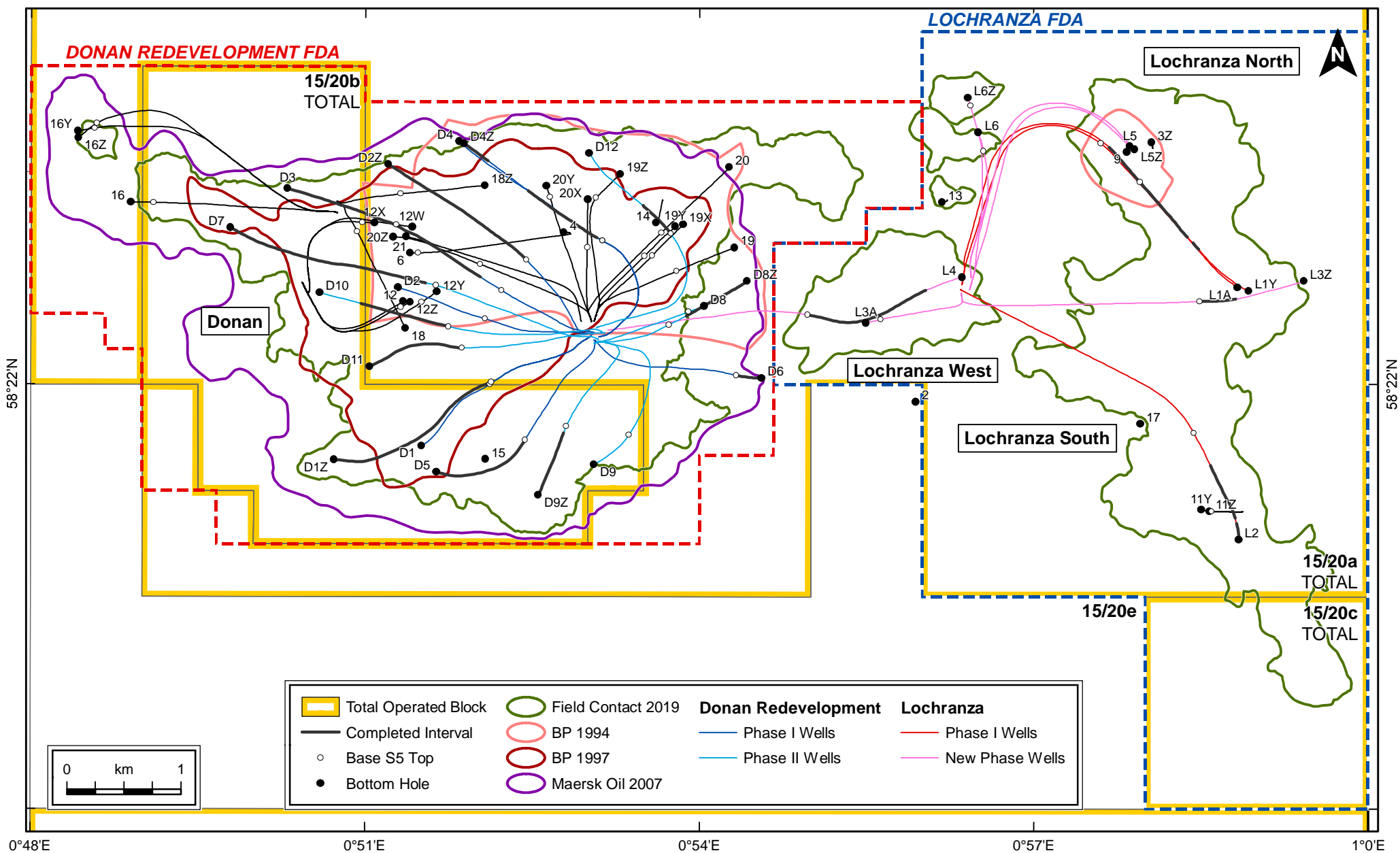
Supplementary material 7. Donan Field outline evolution with time, as a result of improving data quality, additional data points, greater technical insights and associated collapsing of the subsurface uncertainties.
