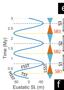
Model Run 22: eustatic control
