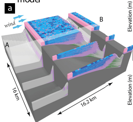
Model Run 21: base model
