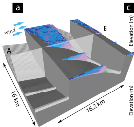
Model Run 24: wind direction
