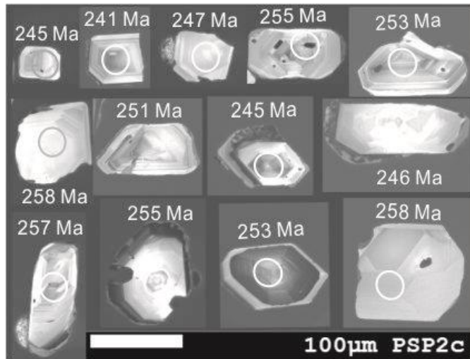
Figure S1. Combined LA-ICP-MS dating results and CL-images of Permian rocks
