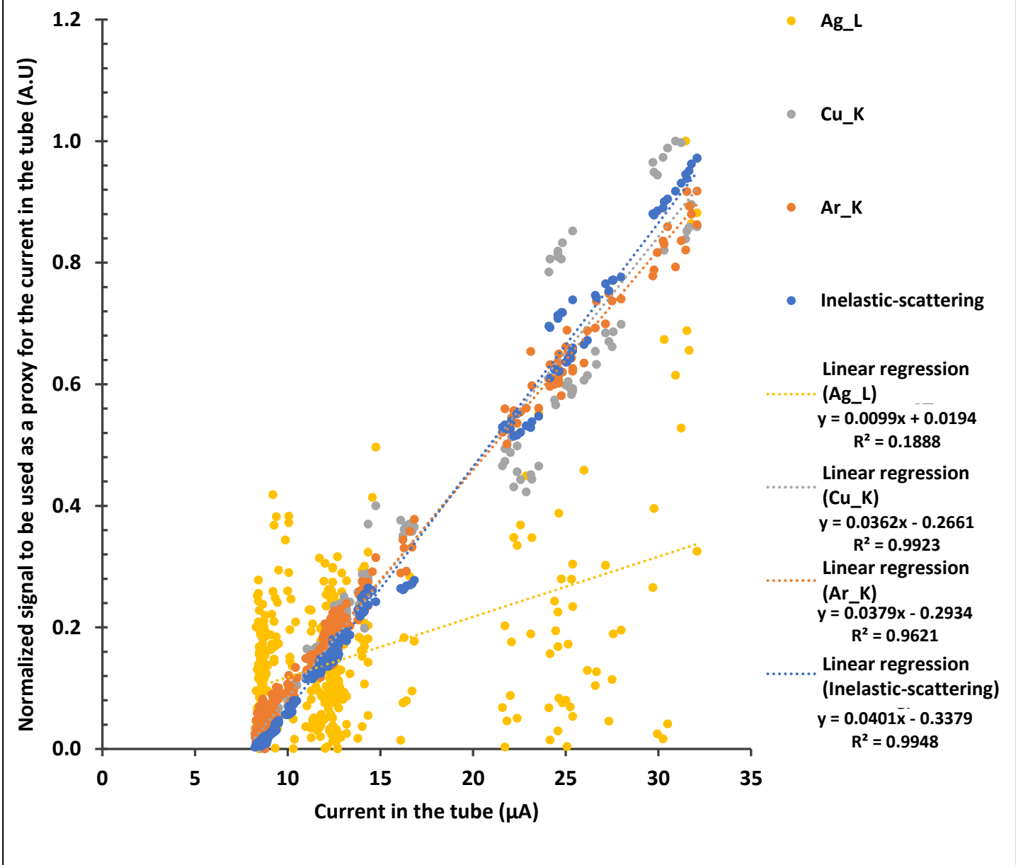
Figure C: Estimation of the tube current using several types of signal normalisation: Ag in L electron shell, Cu in K electron shell, Ar in K electron shell and inelastic-scattering. These can be used as proxies for the current in the tube.
