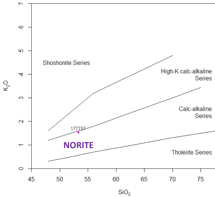
SiO 2 -K 2 O plot (Peccerillo and Taylor 1976)
