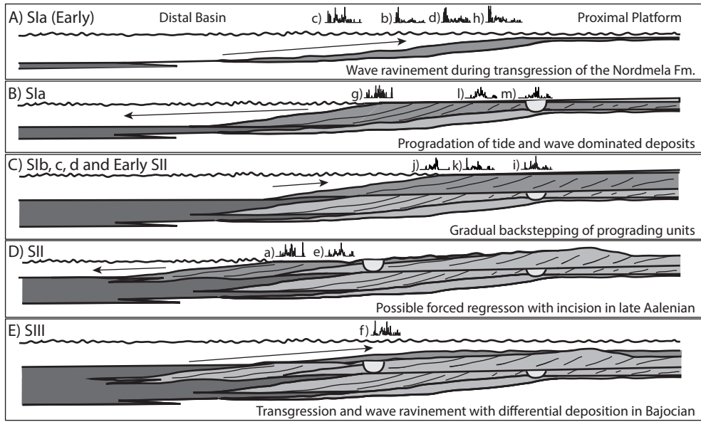
Supplementary Figure S3: Conceptual understanding of the evolution of the parasequences in the Stø Formation. Modified from Gjelberg et al. (1987).
