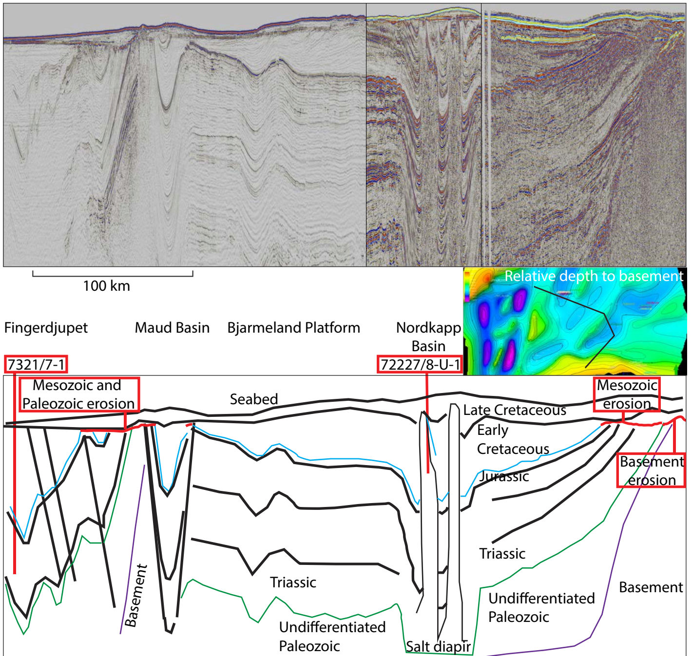
Supplementary Figure S6: Regional north-south seismic cross section across the study area which shows the southern exposure of basement rocks and erosion in the Jurassic. Coarse grained deposits found in the southern wells are derived from this crystalline basement protolith. Inset map shows the depth to basement, and thereby the possible locations for intrabasinal basement exposure. Location of profile is given in inset figure with relative depth to basement.
