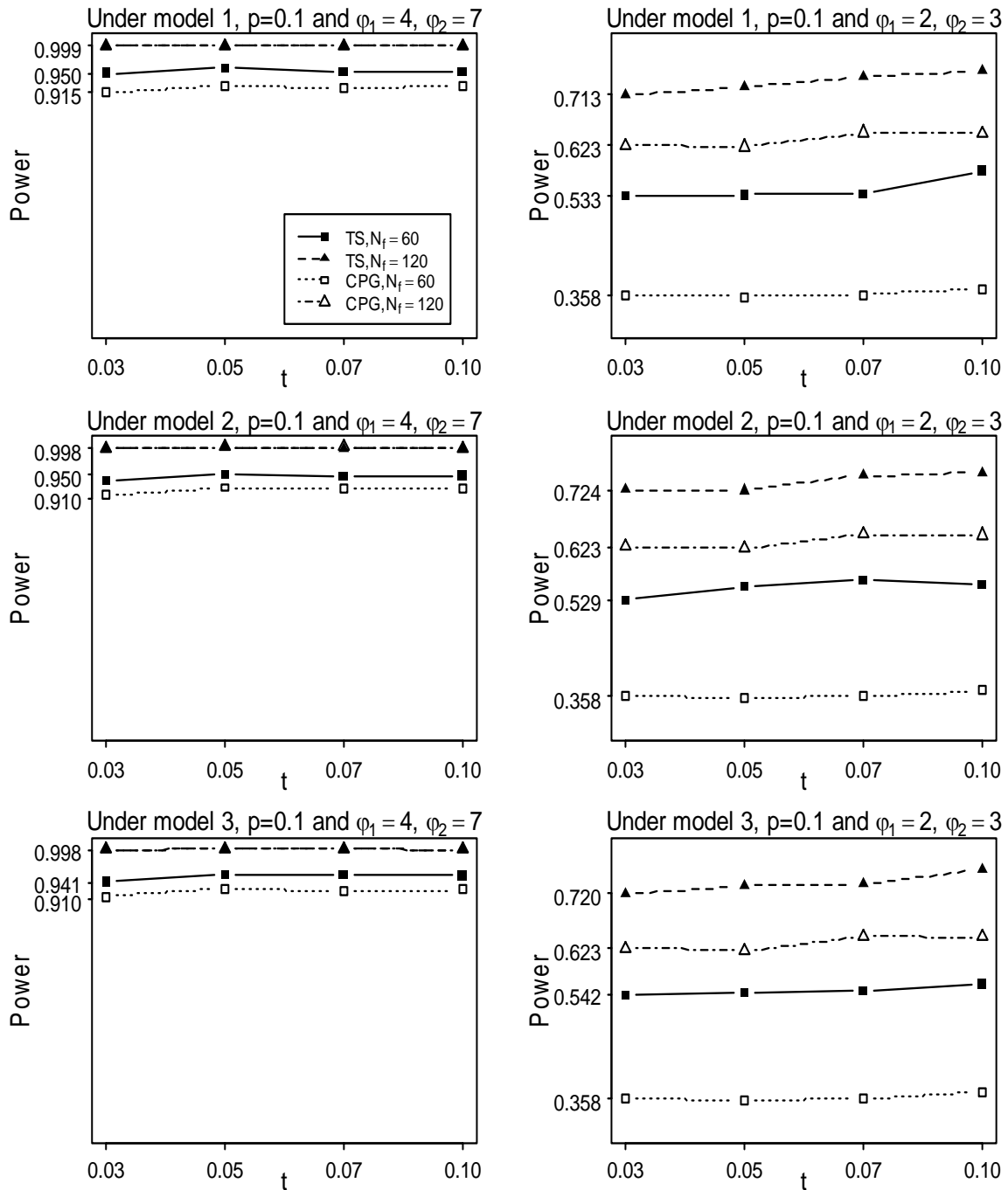
Figure 6. Empirical powers of the TS and CPG tests under p=0.1 , additive genetic model and different levels of population stratification.
