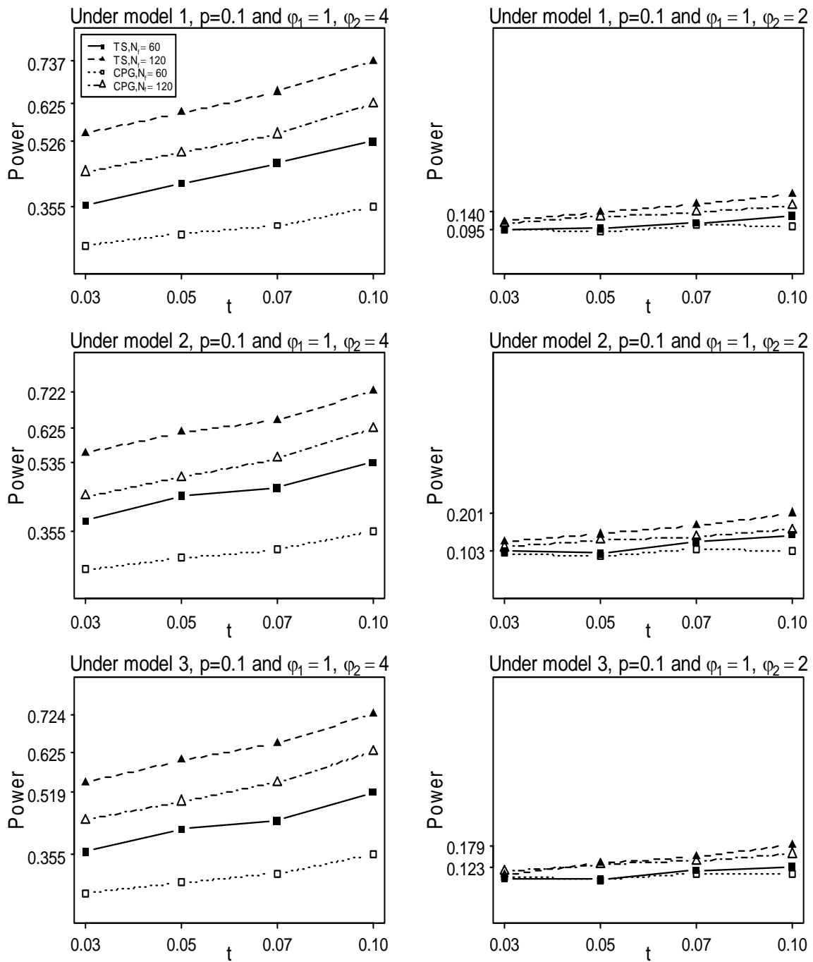
Figure 4. Empirical powers of the TS and CPG tests under p=0.1 , recessive genetic model and different levels of population stratification.
