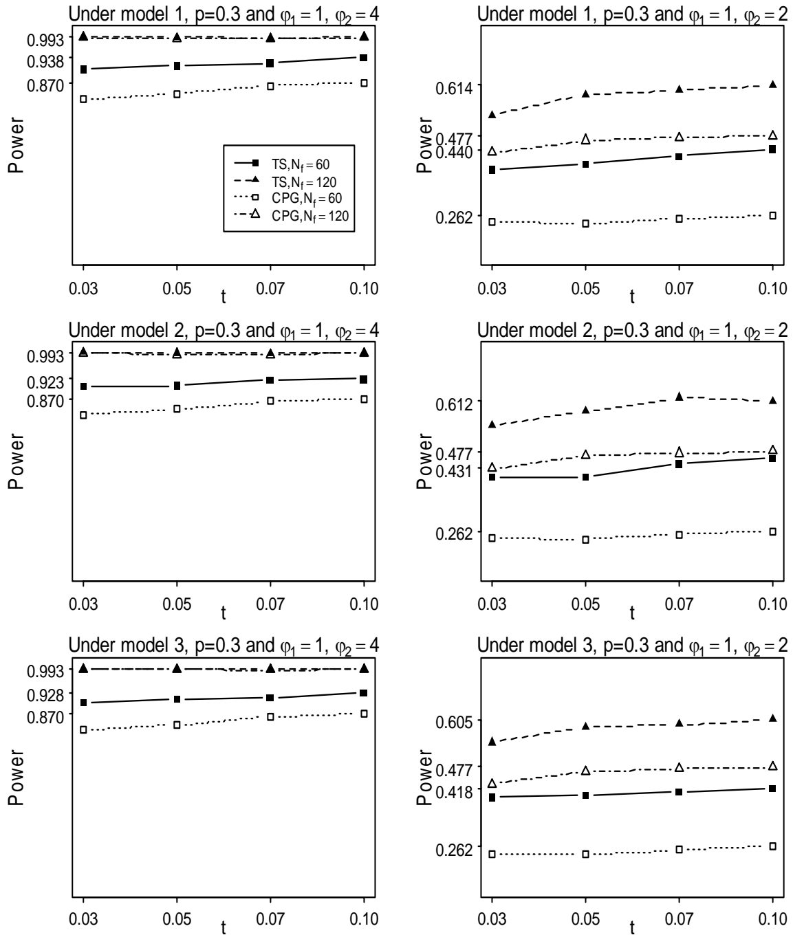
Figure 5. Empirical powers of the TS and CPG tests under p=0.3 , recessive genetic model and different levels of population stratification.
