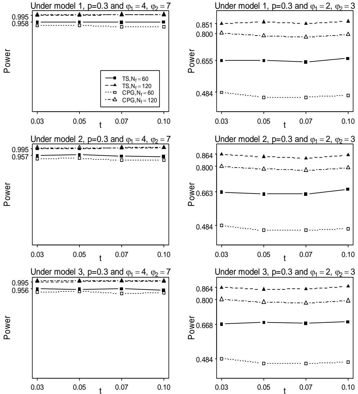
Figure7. Empirical powers of the TS and CPG tests under p=0.3 , additive genetic model and different levels of population stratification.
