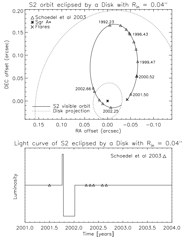
Fig. 3. Same as Fig. 2, but for a disk with inner radius of 0.04'' , R_{\text{out}} = 0.2'' , i = 39^\circ and \beta = 347^\circ . Note that S2 is seen through the hole in early 2002 and that there are no constraints on the disk outer radius in this case.
