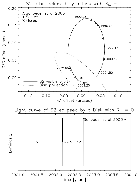
Fig. 2. The orbit (top panel) and the light curve (bottom) produced by S2 passing through a disk with inner radius R_{\text{in}} = 0 and outer one R_{\text{out}} = 0.1'' , i = 71^\circ and \beta = 46^\circ . Triangles show the positions of the star as given by Schödel et al. (2003). Respective times of the observations are shown in the figure for some of the measurements. The two small crosses mark the points where the star would actually pass through the disk and when X-ray and NIR flares are emitted. The S2 luminosity in the bottom panel is shown schematically, in arbitrary units.
