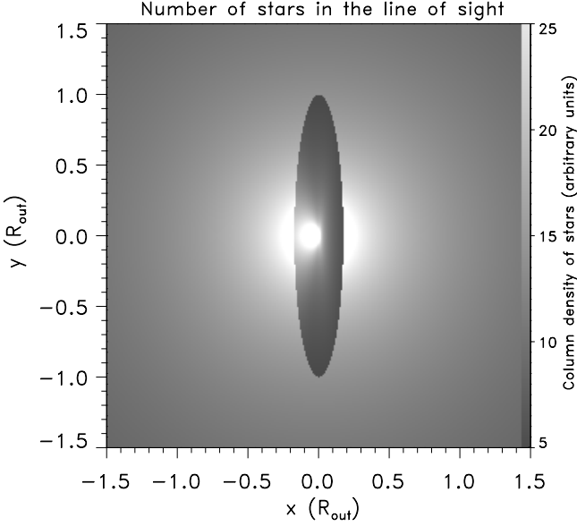
Fig. 13. Image of the star cluster shaded by a disk with inclination angle i = 80^\circ . The brighter areas correspond to larger line of sight column density of stars (the scale is shown on the right of the figure).
