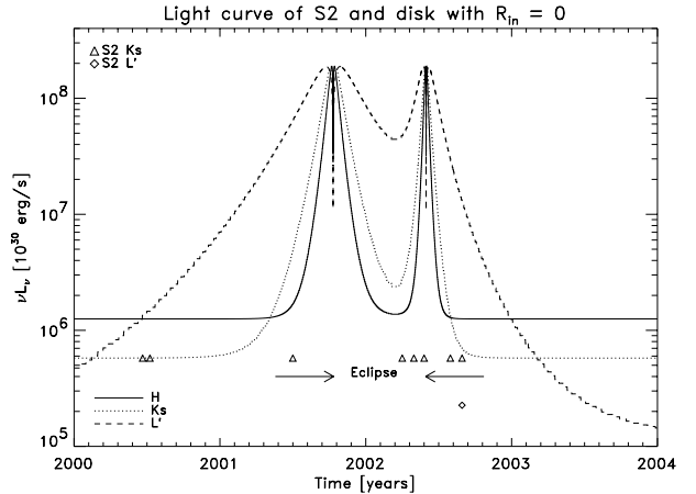
Fig. 7. NIR light curves of S2 and the disk reprocessed emission for i = 60^\circ and \beta = 300^\circ . The triangles show the epochs in which Schödel et al. (2002, 2003) observed this star. The corresponding “observed” stellar luminosity is the model spectral luminosity in the K _s band calculated as explained in Sect. 3.1.1. The diamond shows the model spectral luminosity of S2 plus the excess in the L’ band as observed (Genzel et al. 2003; note that there exists only one detection of S2 in L’ band so far).
