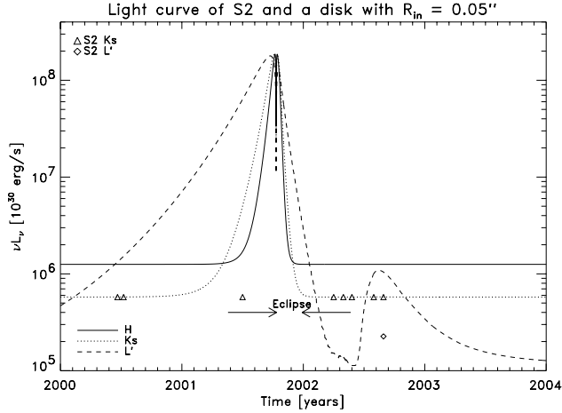
Fig. 11. Same as Fig. 7 but for a disk with an inner hole of R_{\text{in}} = 0.05'' . Note the absence of the second maxima in the H and K_s bands. However the L' band excess is still much larger than observed.
