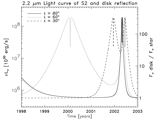
Fig. 9. Model spectral luminosity of S2 plus the disk reemission at 2.2 \mu\text{m} as a function of time for disks with \beta = 80^\circ and different inclination angles. R_{\text{in}} = 0 for this figure.
