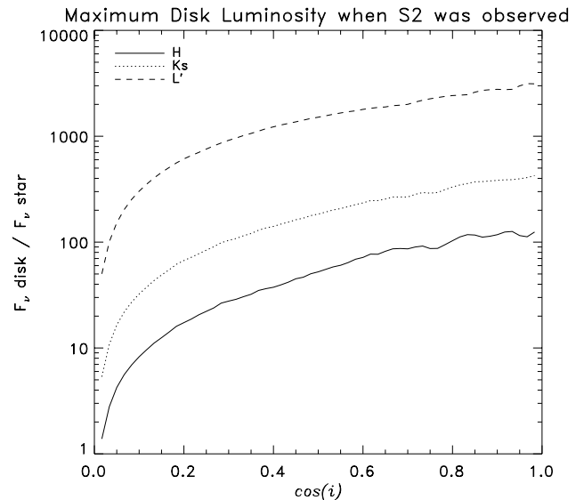
Fig. 10. Maximum spectral luminosity of the disk in the three NIR bands that should have been detected by Schödel et al. (2003) if an optically thick disk with R_{\text{in}} = 0 was present in Sgr A*. The luminosity is shown in units of S2 spectral luminosity as a function of the disk inclination angle. Note that the disk is always much brighter than the star in the infrared except for the nearly edge-on orientation.
