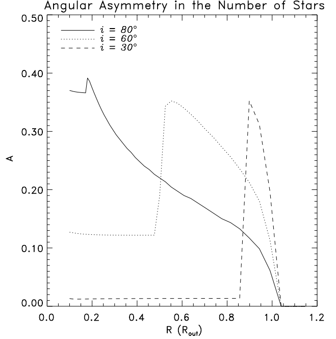
Fig. 14. Anisotropy measure for a “small” disk ( R_{\text{out}} \ll R_{\text{cusp}} ) and three values of the disk inclination angle, i = 80^\circ (solid line), 60^\circ (dotted) and 30^\circ (dashed).
