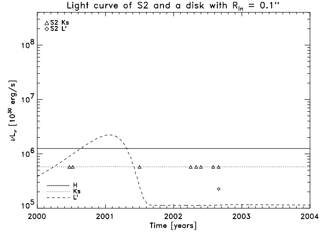
Fig. 12. Same as Fig. 11 but for a larger inner disk hole, R_{\text{in}} = 0.1'' . Note that such a disk does satisfy the observational constraints: there are no eclipses or transient brightening in the K_s band due to disk re-emission of the star’s radiation.
