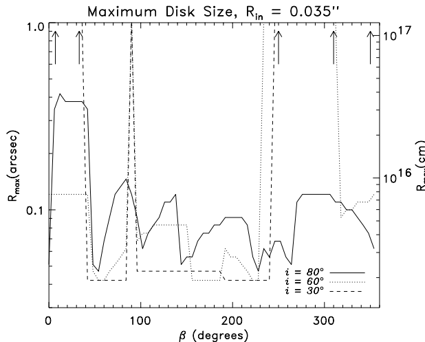
Fig. 4. Maximum disk outer radius for different orientation angles in the case of a disk with inner radius of R_{\text{in}} = 0.035'' . The maximum value of R_{\text{out}} is shown as a function of the rotation angle for three different values of the inclination angle (labelled in the figure). The curves are not smooth because the number of the observed S2 positions is finite; had we had a full continuous coverage of S2 orbit from 1992 to 2002, the respective curves would become smooth functions. Vertical arrows at the top of the plot emphasize the fact that the outer disk radius can be arbitrarily large for the respective set of parameters. In general much larger disks are allowed if R_{\text{in}} \gtrsim few tens of a milli-arcsecond.
