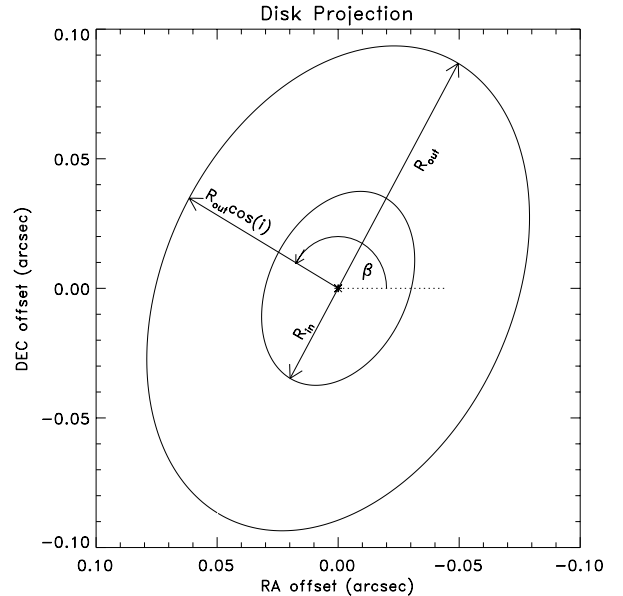
Fig. 1. Projection of the disk in the plane of the sky. The disk is described by two radii, R_{\text{in}} and R_{\text{out}} , and two angles: disk inclination angle, i , and rotation angle, \beta . The latter is defined as the angle between the West projection and the semi-minor axis of the disk projection directed to the part of the disk closest to the observer.
