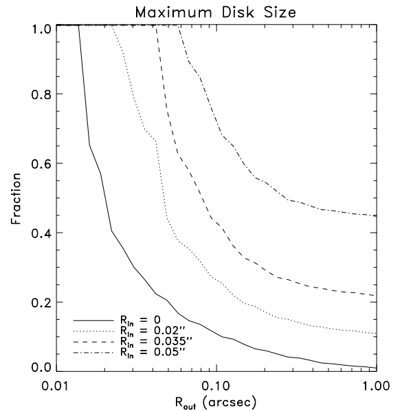
Fig. 5. Fraction of the parameter space that permits a disk of a given R_{\text{out}} . The curves are for different values of R_{\text{in}} as marked in the figure legend.
