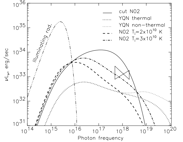
Fig. 1. The up-comptonized emission of the close star S2 during its closest approach to Sgr A* in 2002 for five different accretion flows, as marked in the figure. The spectrum of the star illuminating the inner 100 Schwarzschild radii of the flow is also shown for comparison. The Chandra data with uncertainties (Baganoff et al. 2003) are shown with the bow-tie.
