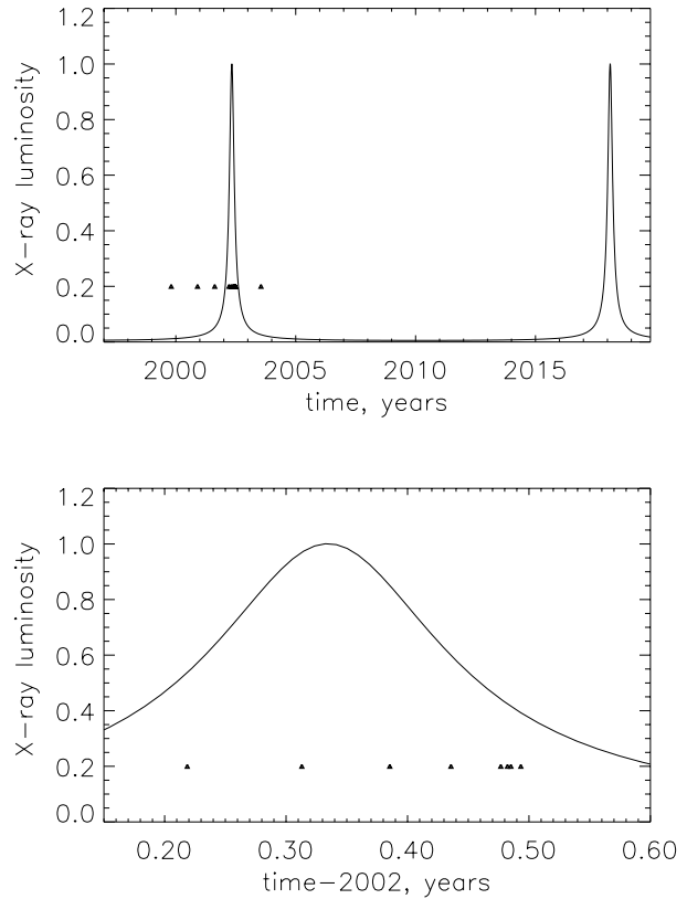
Fig. 2. The lightcurve of the optical/UV radiation of the close star S2 up-comptonized by the accretion flow into the X-ray band. The upper panel shows the lightcurve on time scales of tens of years, while the lower one shows the emission during 2002 when S2 passes through the pericenter of its orbit. The filled triangles mark the epochs when Chandra observed the Galactic Center region (Park et al. 2004; Eckart et al. 2004). The y -coordinate of the triangles in the figure is arbitrary.
