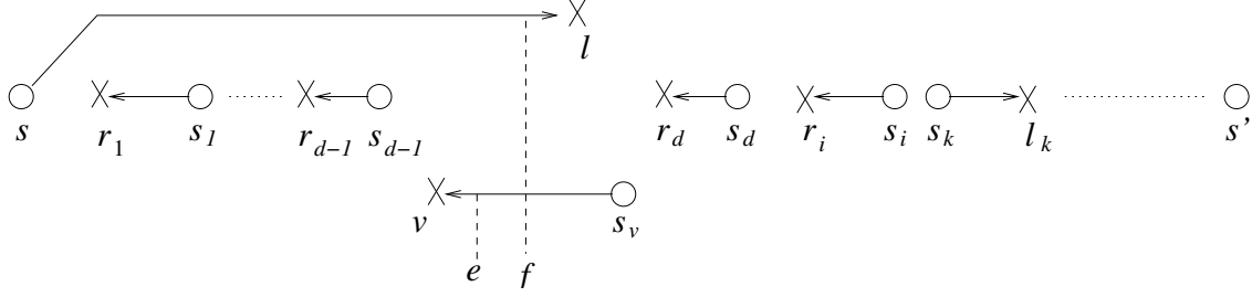
Figure 4: The situation considered in Lemma 7. Note that the interval (v, e) has been erased by other requests (descendants of r_d ) that are not shown in this figure, whereas the interval (f, \ell) does not get erased because it was protected by left requests that are not shown. Of course, v = e and f = \ell (and/or f = s_v ) are possible, as well as v = r_d (instead of a descendant of r_d ).
