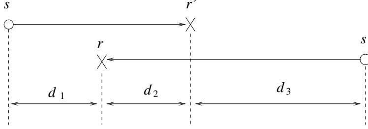
Figure 3: The situation considered in Lemma 6.
