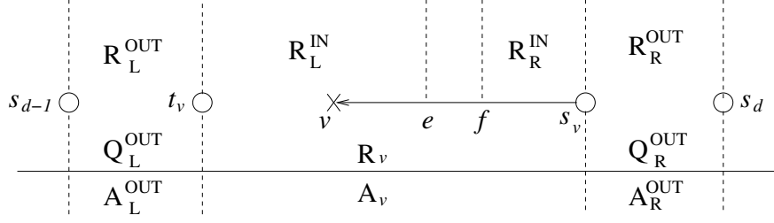
Figure 5: Zooming in on request v and what happened afterwards. Compare Figure 4.
