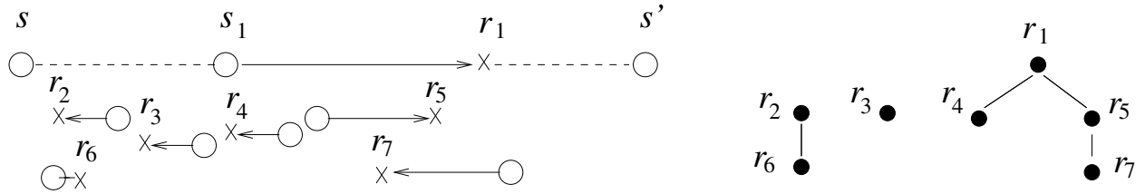
Figure 2: An example forest. Request r_i is served by server s_i ( i = 1, \dots, 7 ). The roots are r_2, r_3, r_1 , forming the word RRL . The children of r_1 form the word RL . Note that r_3 arrived before r_2 ; if it had not, s_2 would have already been used when r_3 arrived, and in our construction r_3 would have become a root of a tree in the interval (s, s_3) , with r_2 as its child.
