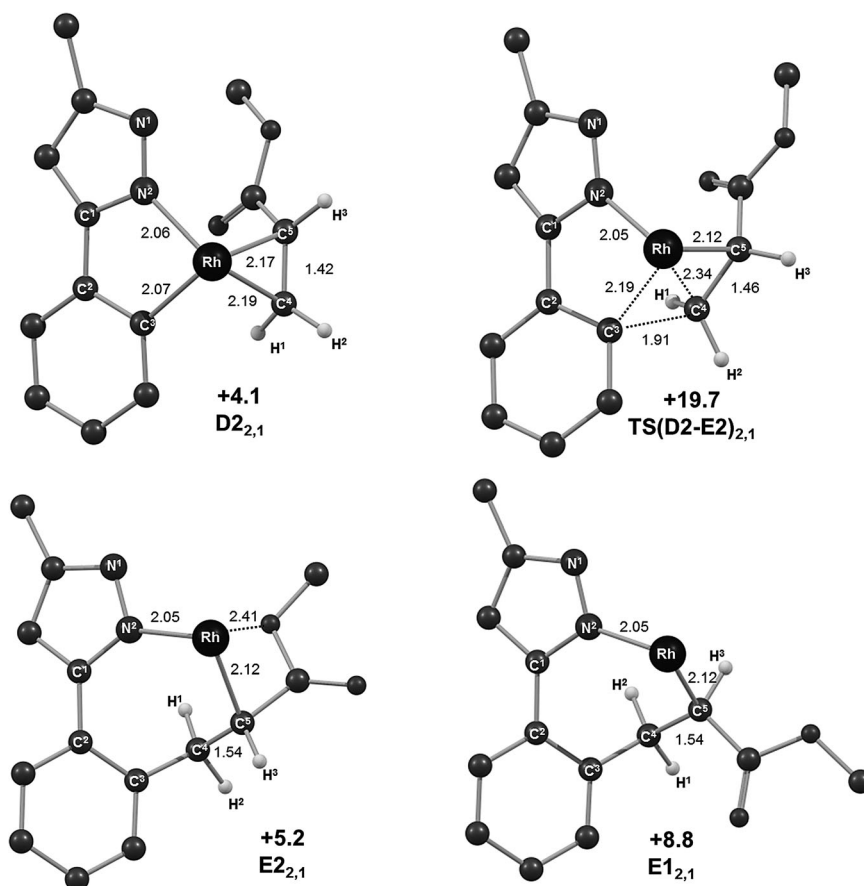
Figure 3. Computed structures for 2,1-insertion starting from D2_{2,1} with relative energies in kcal mol -1 and selected distances in Å. The geometry of E1_{2,1} is included for comparison. The Cp* ligand (which lies above the plane of the page) and all hydrogen atoms except those on C4 and C5 have been omitted for clarity.
