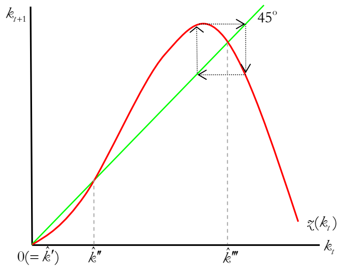
Figure 3. \nu = 0 and z'(k_t^3) < -1 : an example with a period-2 cycle
