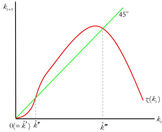
Figure 2. \nu = 0 and -1 < z'(\hat{k}''') < 0
