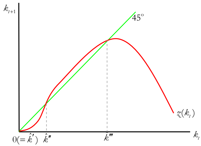
Figure 1. \nu = 0 and 0 < z'(k''') < 1
