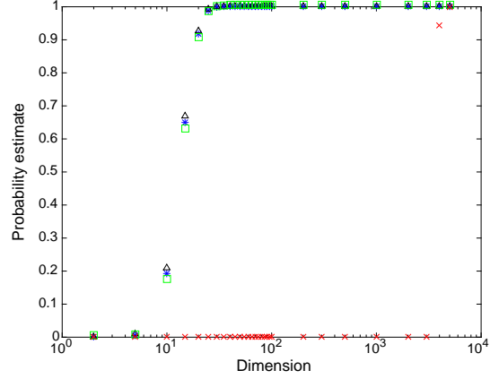
Figure 2: Estimates of probabilities that a random point in a sample of 20000 points i.i.d. drawn from an equidistribution in the unit cube [0, 1]^n in \mathbb{R}^n is separable from the remaining points in the sample as a function of dimension n . Blue stars, black triangles, and green squares, are the means, maxima, and minima of N_-/N over all 100 samples for each value of n . Red crosses show estimates (12).
