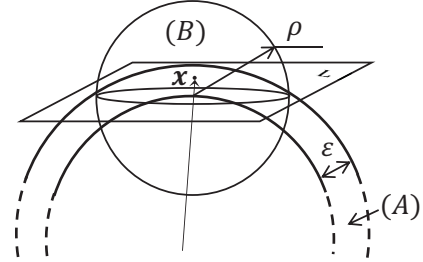
Figure 1: Point \mathbf{x} belongs to a spherical layer (A) of thickness \varepsilon . The data are centralized and the centre of the spheres from A is the origin. Hyperplane L is orthogonal to vector \mathbf{x} and tangent to the internal sphere of A . L cuts an upper spherical cap from A and separates \mathbf{x} from the data points which belong to the external sphere of A but do not belong to that cap. The cap is included into the upper half of ball (B) . The centre of B is intersection of the radius x with the internal sphere of the layer A .
