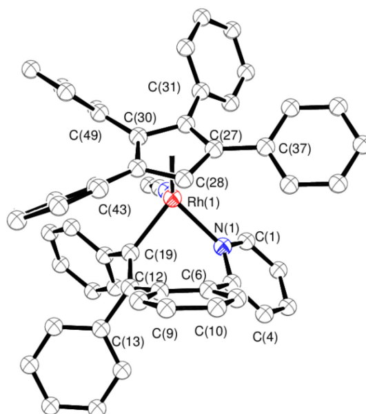
Figure 4 Molecular structure of the cation of 5b hydrogen atoms are omitted for clarity; ellipsoids are set at 50% with selected bond lengths (Å). Rh(1)-C(19) 2.076(3), Rh(1)-N(1) 2.123(3), Rh(1)-C(26) 2.268(3), Rh(1)-C(27) 2.284(3), Rh(1)-C(28) 2.157(3), Rh(1)-C(29) 2.213(3), Rh(1)-C(30) 2.187(3).
