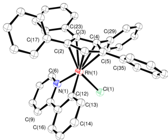
Figure 3 Molecular structure of 2 hydrogen atoms are omitted for clarity; ellipsoids are set at 50%, with selected bond lengths (Å), Rh(1)—C(1) 2.139(2), Rh(1)—C(2) 2.172(2), Rh(1)—C(3) 2.316(2), Rh(1)—C(4) 2.291(2), Rh(1)—C(5) 2.173(2), Rh(1)—C(12) 2.019(2), Rh(1)—N(1) 2.063(2).
