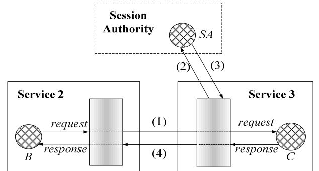
Fig. 5. Protocol 2: Authenticating a session partner
