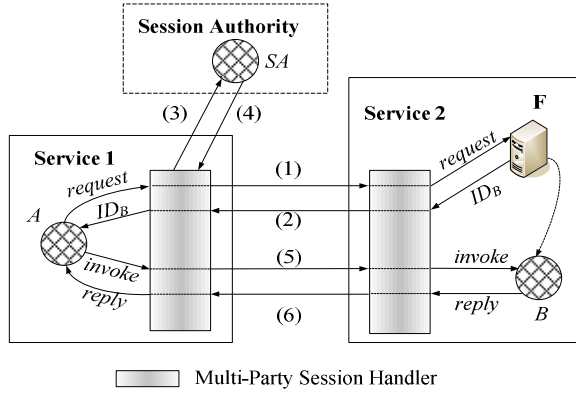
Fig. 4. Protocol 1: Accepting a new session partner
