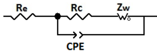
Figure 1. Electrical circuit for analysis of NiMH batteries through EIS
