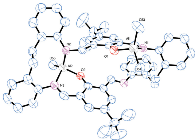
Fig. 3 Molecular structure of [(AlMe)(AlMe_2)L^5] \cdot 2\frac{1}{4}MeCN (7, R = tBu ) (7), with atoms drawn as 50% probability ellipsoids. Hydrogen atoms and MeCN of crystallisation have been omitted for clarity. This is one of two similar macrocyclic complexes in the asymmetric unit. Selected bond lengths (Å) and angles ( ^\circ ): Al1–O1 1.761(4), Al1–N1 1.963(5), Al1–C53 1.977(6), Al1–C54 1.949(5), Al2–O2 1.768(4), Al2–N2 1.860(4), Al2–N3 1.970(4), Al2–C55 1.963(5); O1–Al1–N1 94.49(17), C53–Al1–C54 119.3(3), N2–Al2–N3 110.90(18), O2–Al2–C55 109.2(2).
