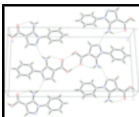
Fig. 2. Perspective view of the crystal packing showing hydrogen-bond interactions (dashed lines). H atoms not involved in hydrogen bonding have been omitted for clarity.
