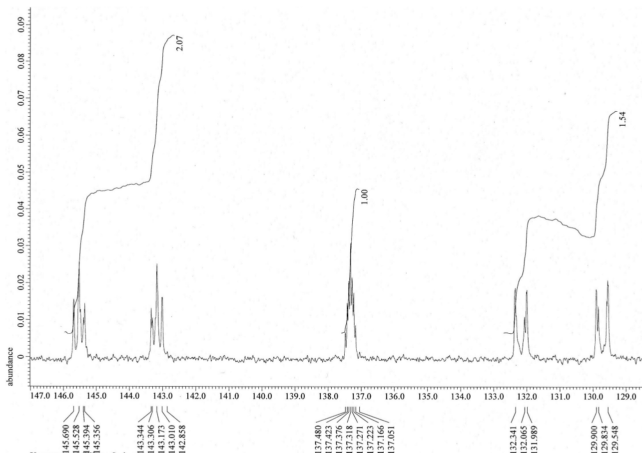
Figure 2-6. C-F coupling in compound 96 : partial ^{13}C NMR spectrum ( CDCl_3 )
